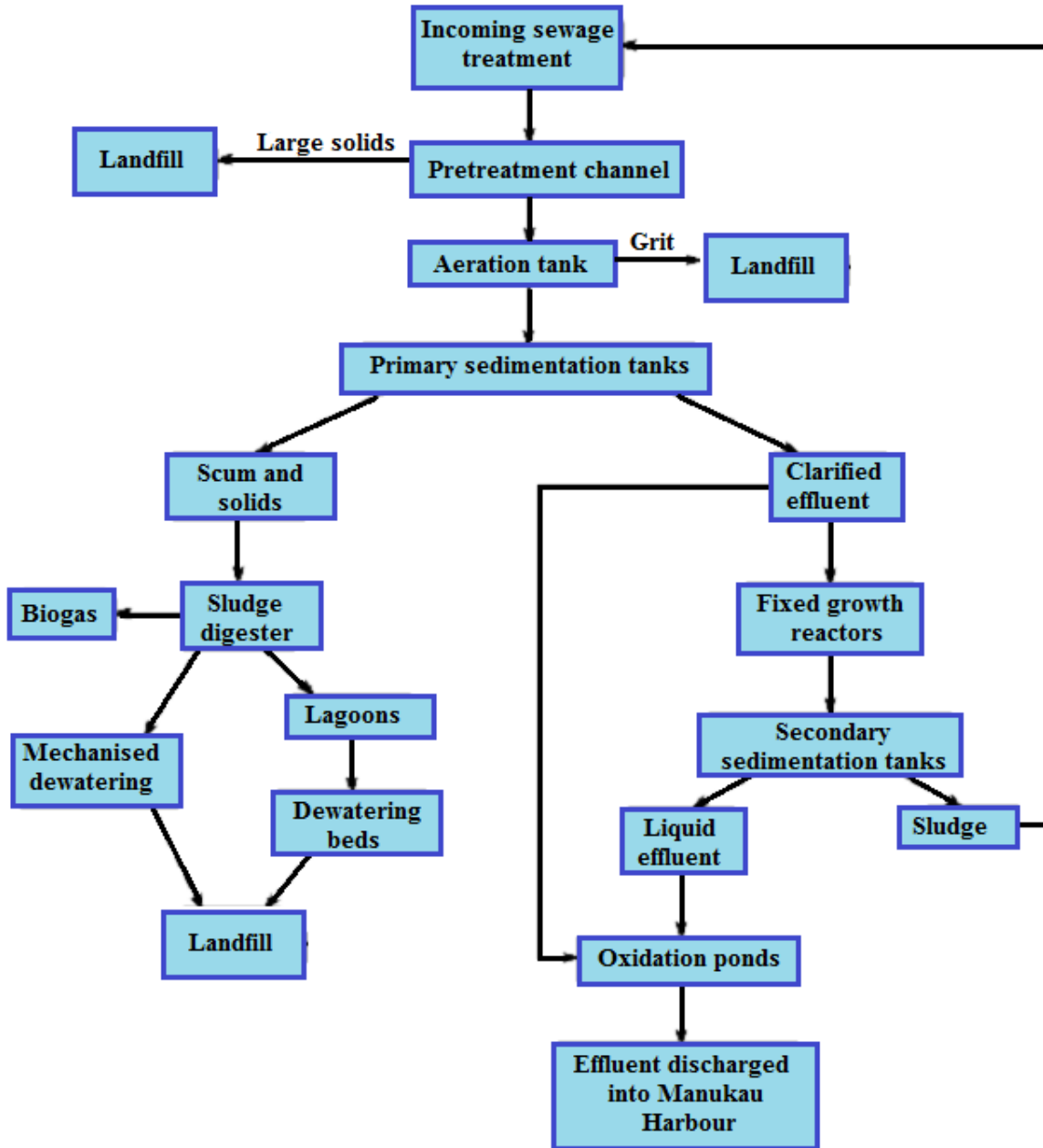
Figure 1: Sewage treatment flow diagram
